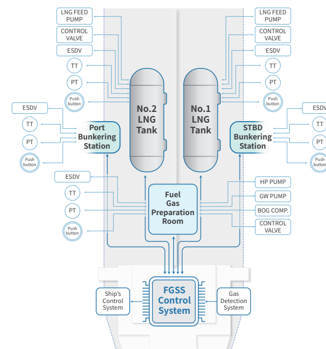
FGSS Control System Logic
